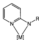
Scheme 1. Aminopyridinato ligand ([M] = early transition metal moiety; R = aryl, silyl or alkyl substituent)
