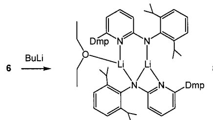
Scheme 8. Synthesis of 8 (Dmp = 2,6-dimethylphenyl)
