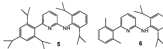
Scheme 2. Ap * H ( 5 ) and Ap ′ H ( 6 )
